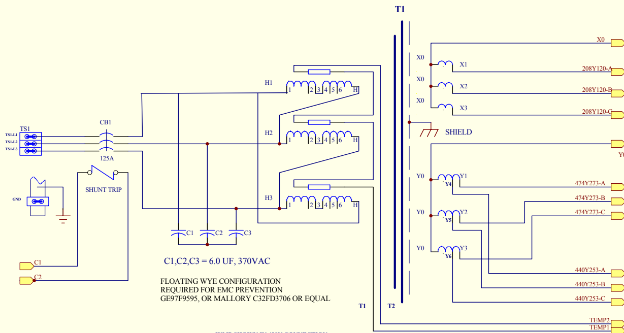
JUMP SHOWN IN 480V CONNECTION
